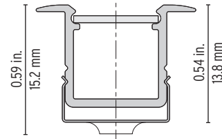
Countersink Clip
